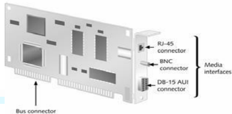
Figure 4-2 Ethernet NIC with interfaces for thinnet (BNC), thicknet (AUI), and 10BaseT (RJ-45)
