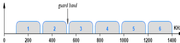
Figure 11.5 A frequency domain plot of the channel allocation from Figure 11.4 with a guard band visible between channels.
