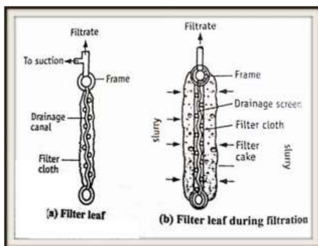
Fig 3 – Filter leaf
