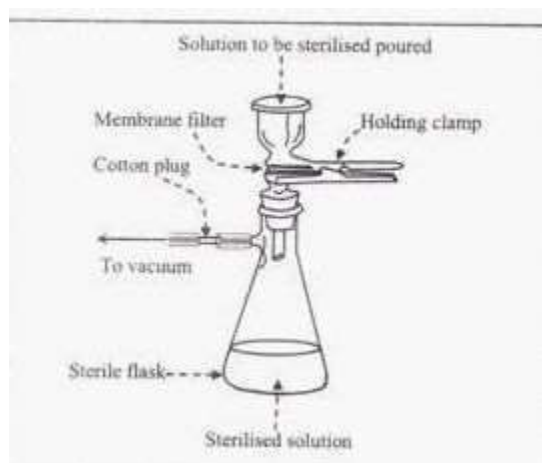
Fig 8- Membrane filter
