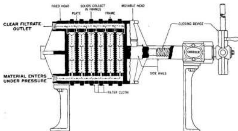
Fig 1- Filter press
