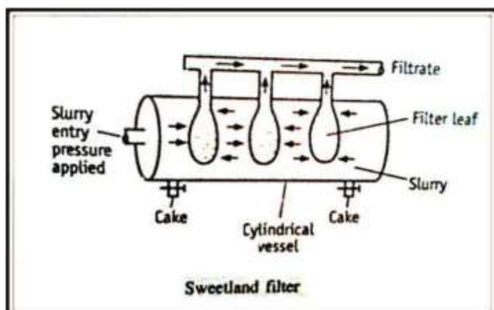
Fig 4 – Sweetland filter
