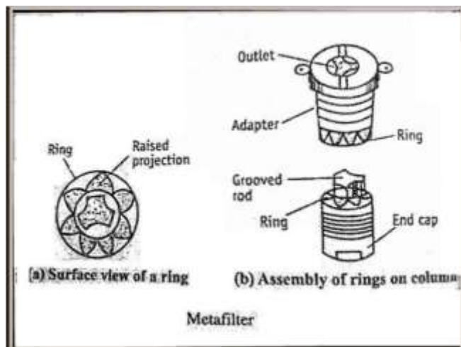
Fig 5 - Metafilter
