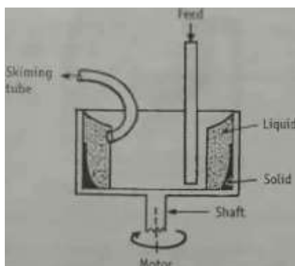
FIG 2-NON-PERFORATED BASKET CENTRIFUGE
