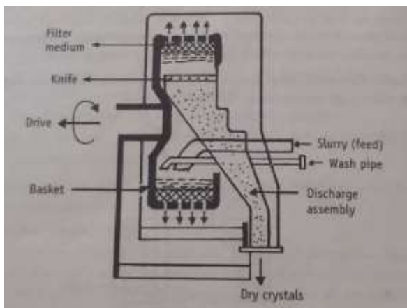
Fig 3 - SEMI-CONTINUOUS CENTRIFUGE
