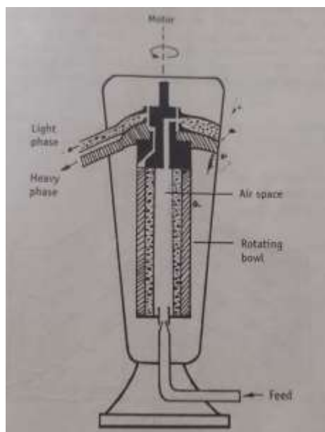
FIG 4 - SUPERCENTRIFUGE
