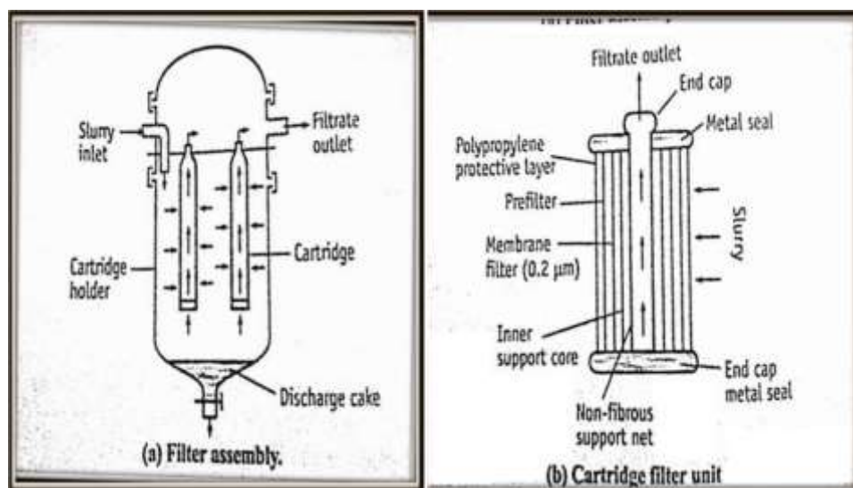
Fig 6 – Cartridge filter
