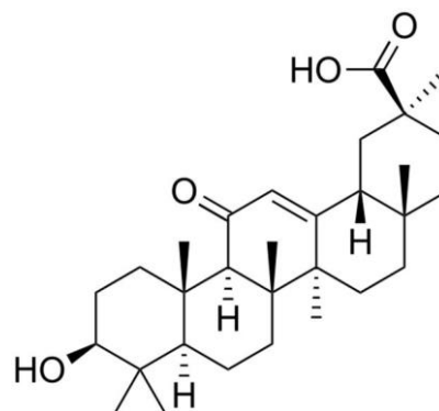
Glycyrrhetic acid
