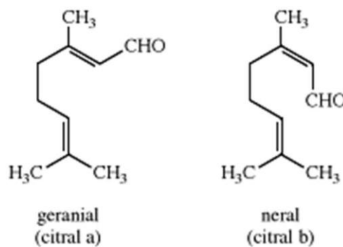
Citral
