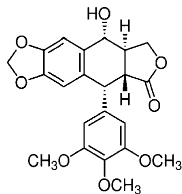
Podophylotoxin
