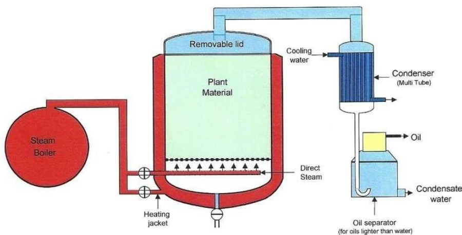
Fig. 3: Steam distillation
